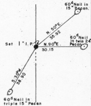
EAST 1/4 CORNER
