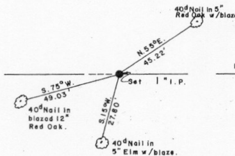
SOUTH 1/4 CORNER
