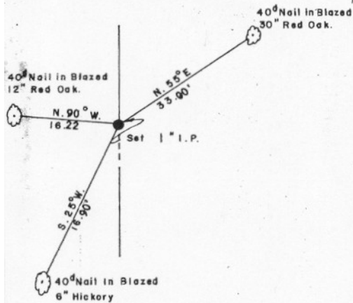
WEST 1/4 CORNER
