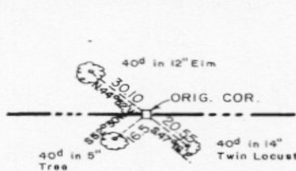
SOUTH 1/4 COR.
