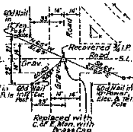
SOUTH 1/4 COR.
