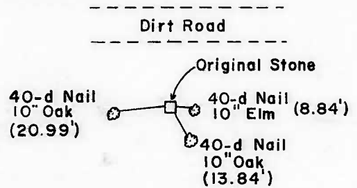
EAST 1/4 CORNER
