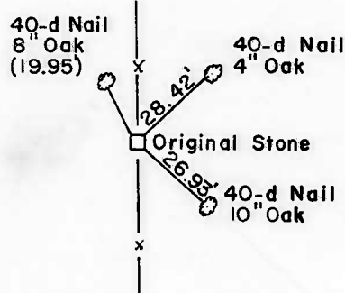
SOUTH 1/4 CORNER
