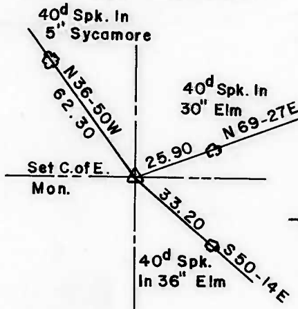
SOUTH 1/4 CORNER
