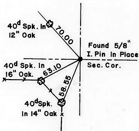
WEST 1/4 CORNER
