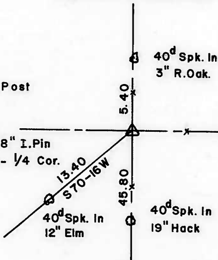
SOUTH 1/4 CORNER
