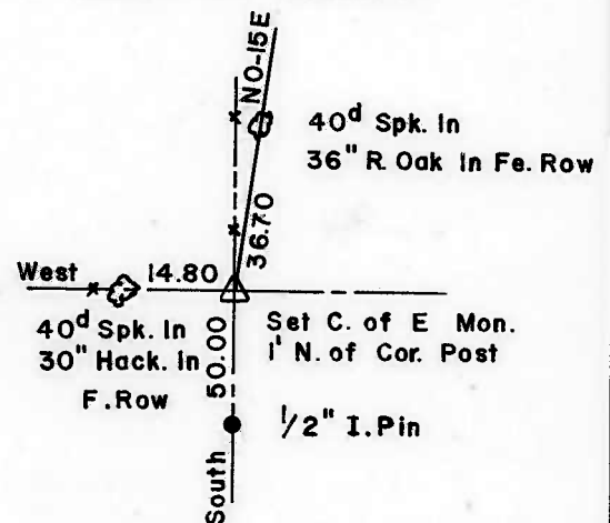
EAST 1/4 CORNER
