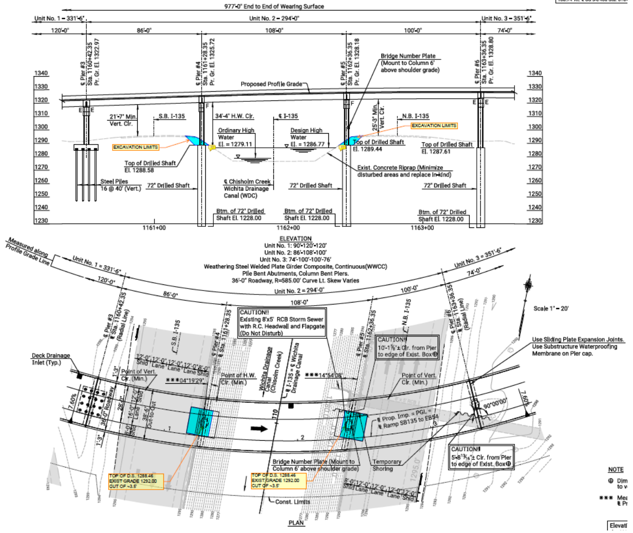
Figure 4: Proposed Pier Locations (from A.M. Cohran & Son, Inc. submitted plans)
