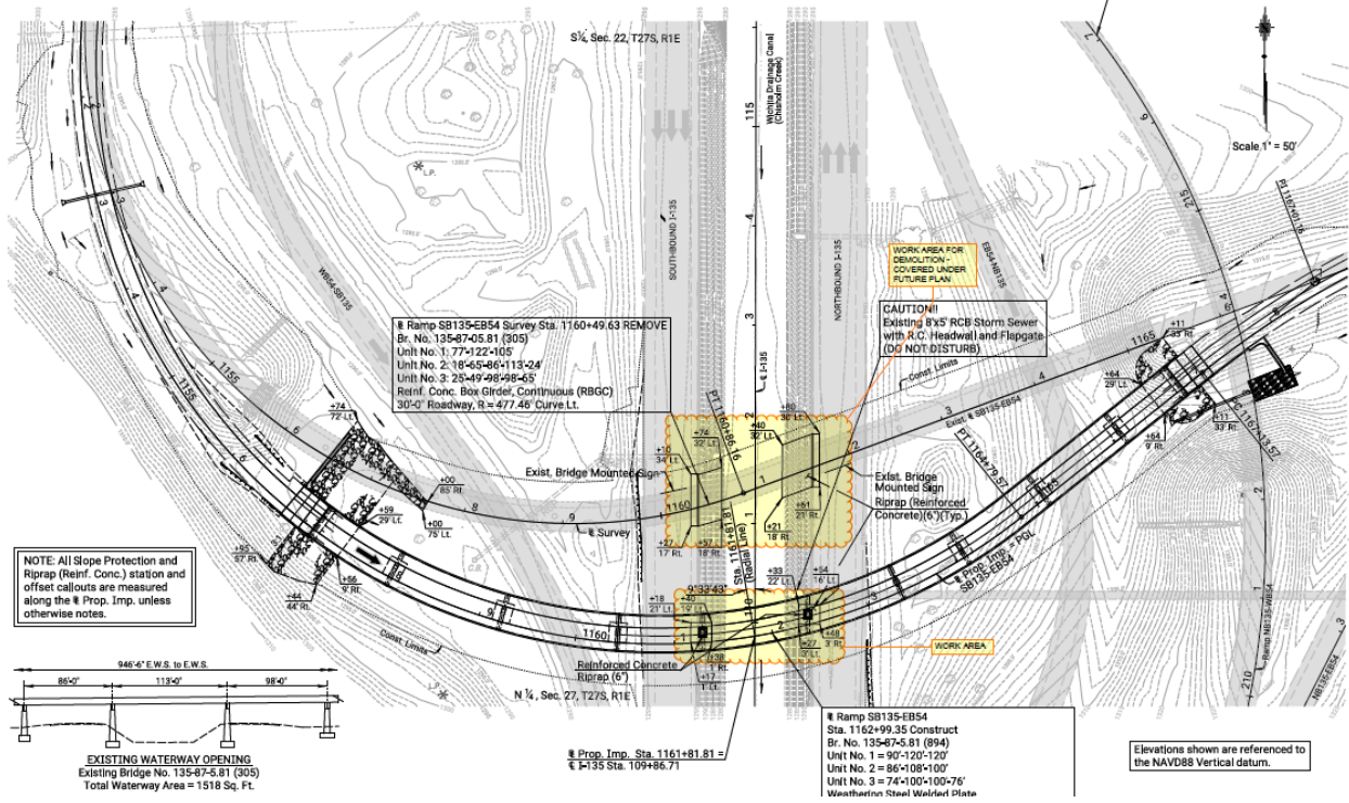
Figure 3: Proposed Bridge Replacement (from A.M. Cohran & Son, Inc. submitted plans)
