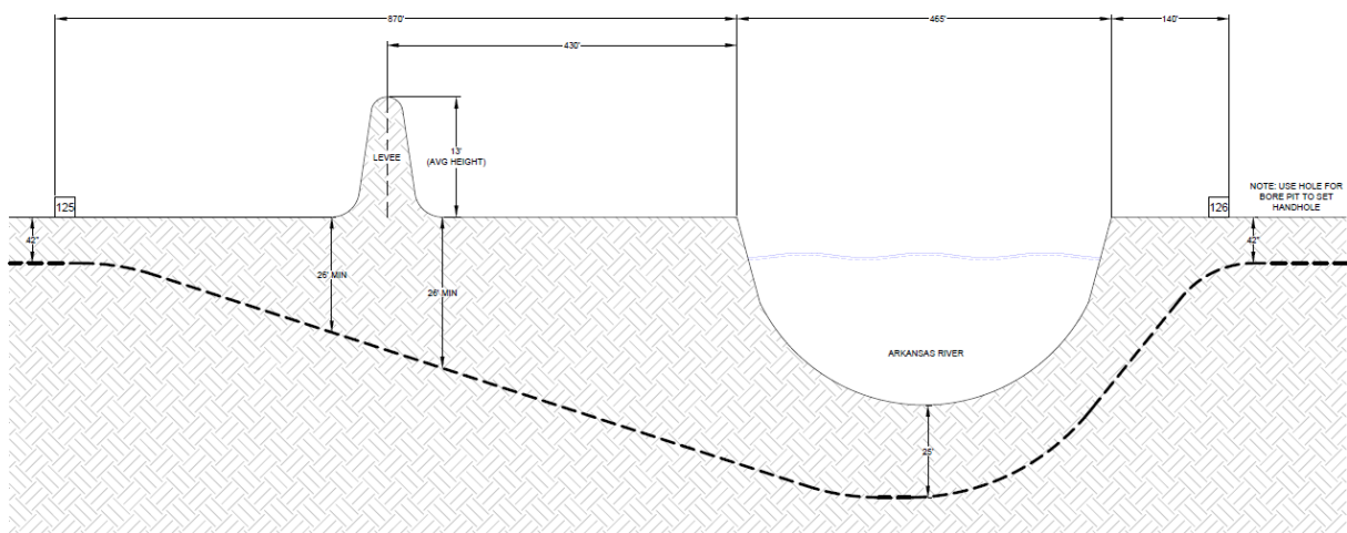
Figure 4: Proposed HDD Bore Profile
